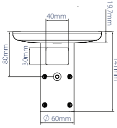
CEILING PLATE - REAR VIEW
