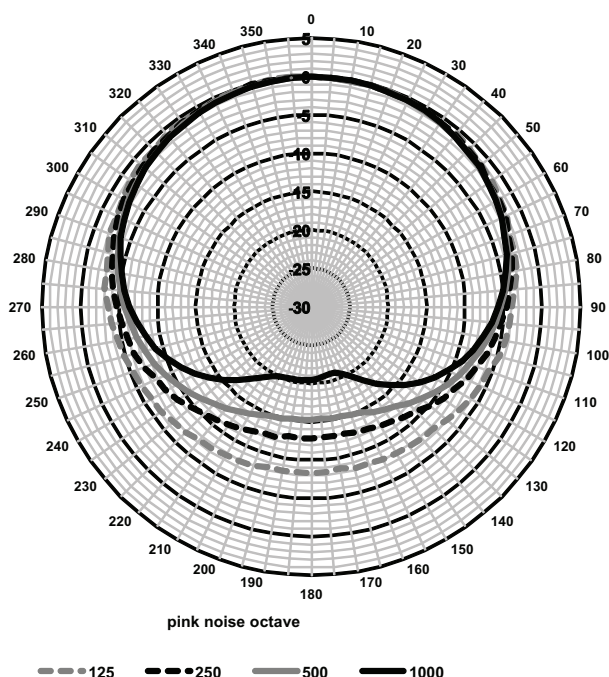
Fig. 2: Polar diagram (measured with pink noise)
