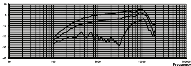
Fig. 1: Frequency response (Opening angle: 0, 90 and 180 degrees)
