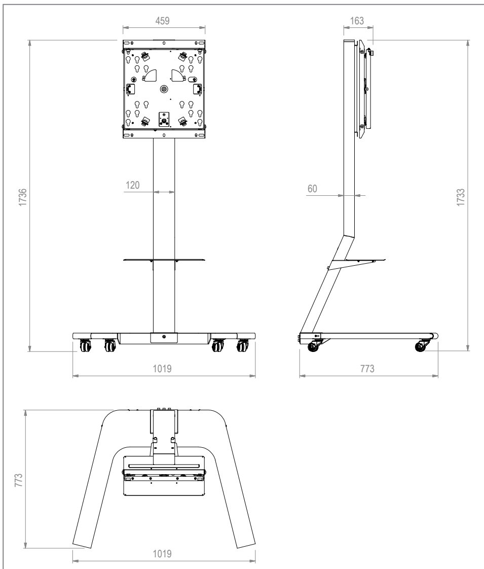
incl. shelf, optionally usable
